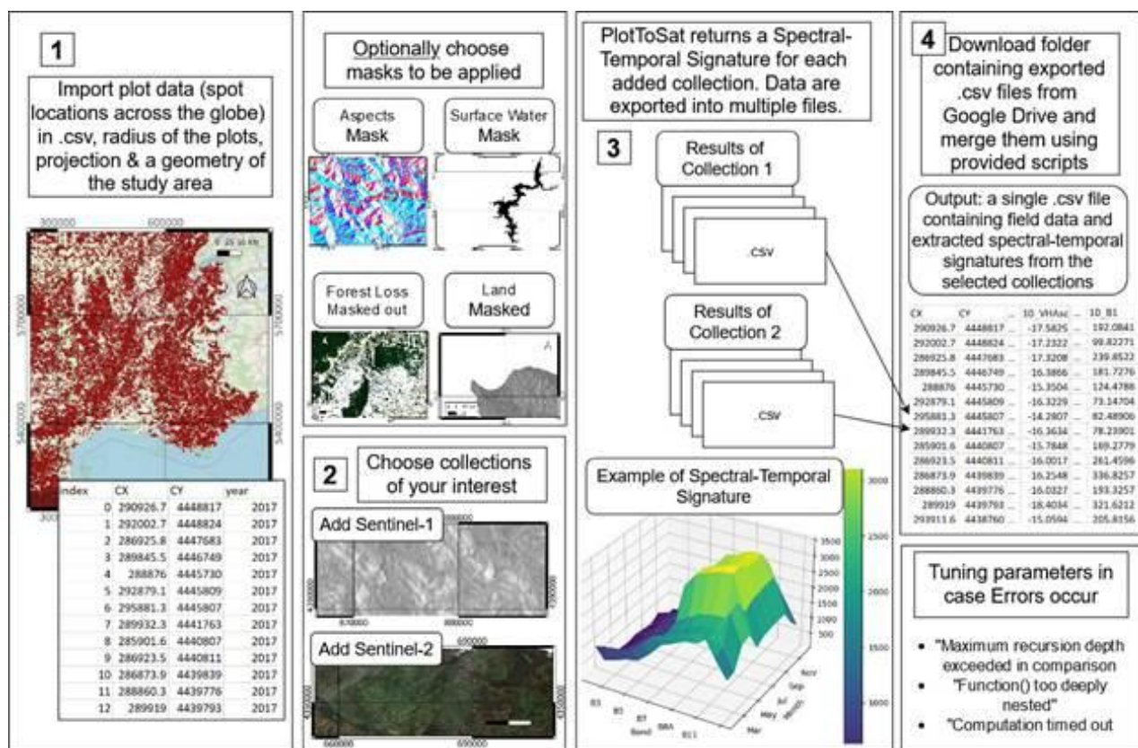
Front-end workflow of the published version of PlotToSat
